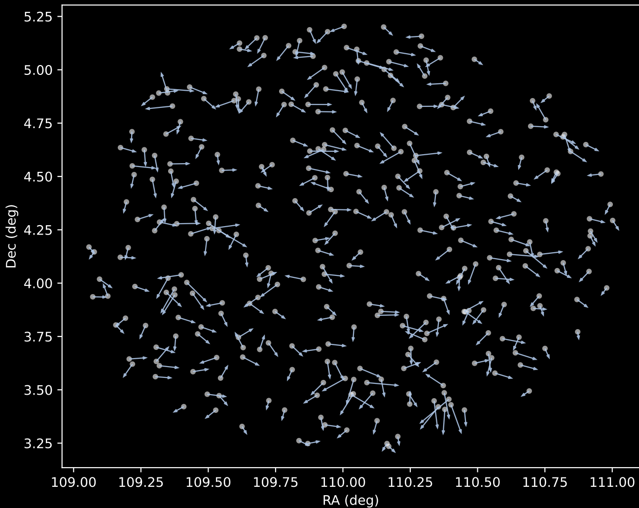
GALAH DR4 Cluster 1 Proper Motion Vectors (n=322)
