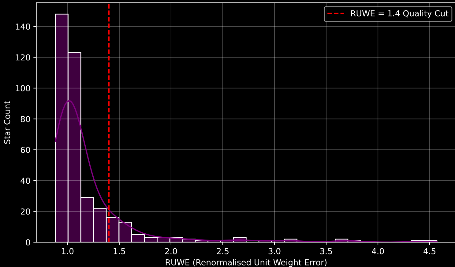
GALAH DR4 Field [6697] RUWE Distribution (n= 382)
