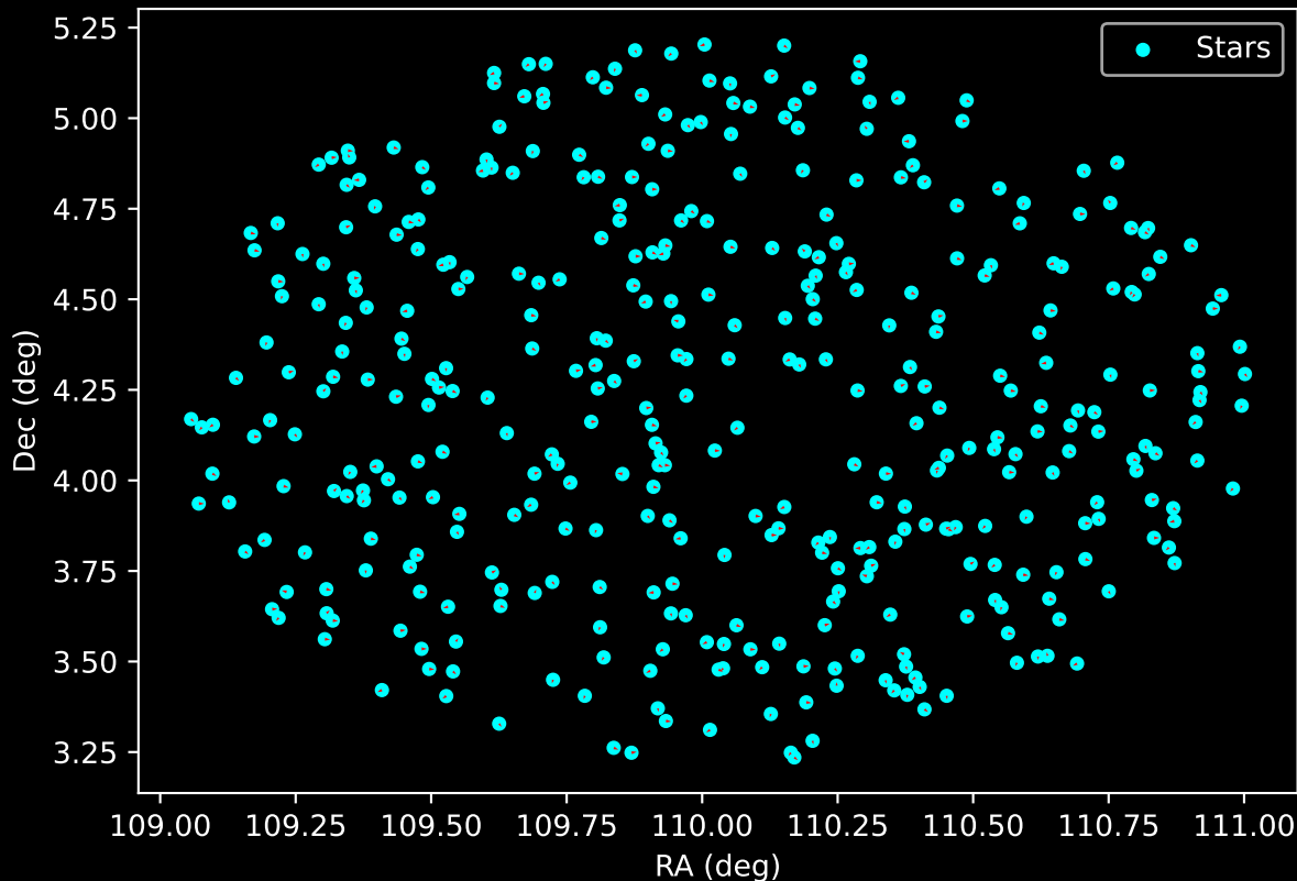
GALAH DR4 Field: [6697] Proper Motion Vectors for Gaia Star Field (n= 394)
