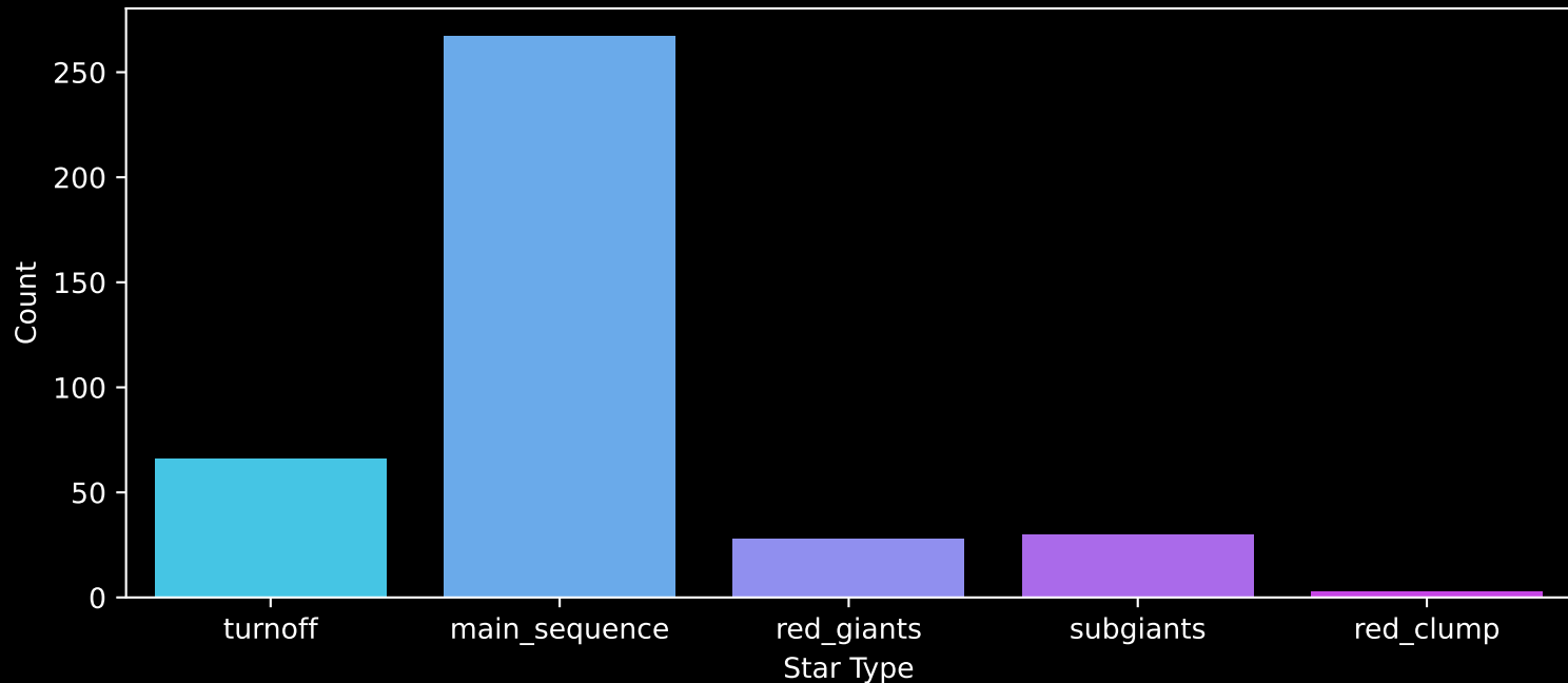
GALAH DR4 Field: [6697] Count plot of Star Type
